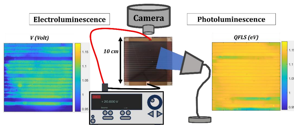
Figure – Hyperspectral luminescence imaging technique (EL and PL) on a 10x10 cm 2 module of 20 cells. Mapping of potential and QFLS from fitting the spectra
